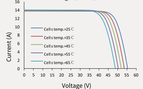
Current-Voltage (615W)
